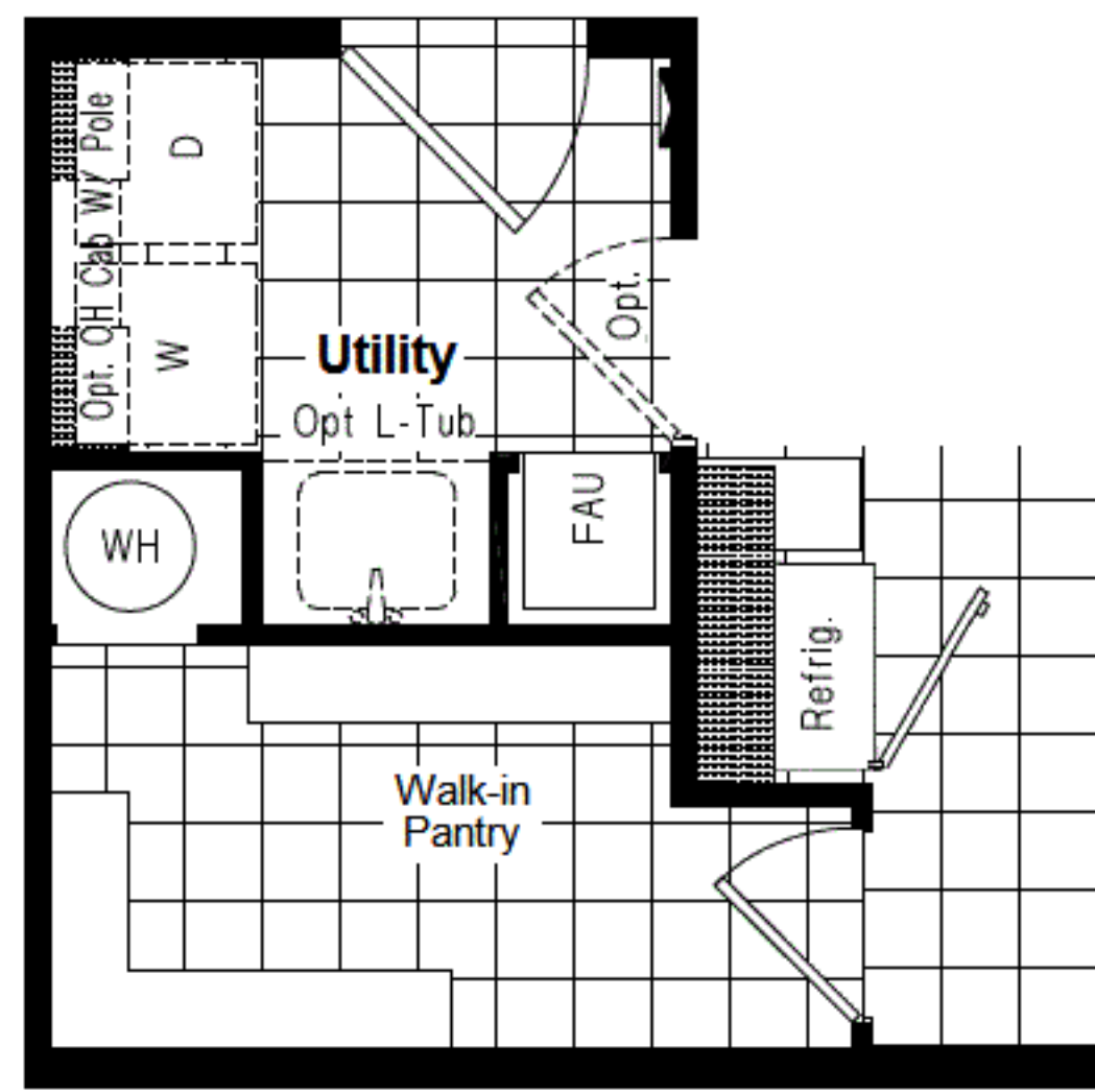
OPT. WALK-IN PANTRY (Only Available w/Standard Kitchen)
