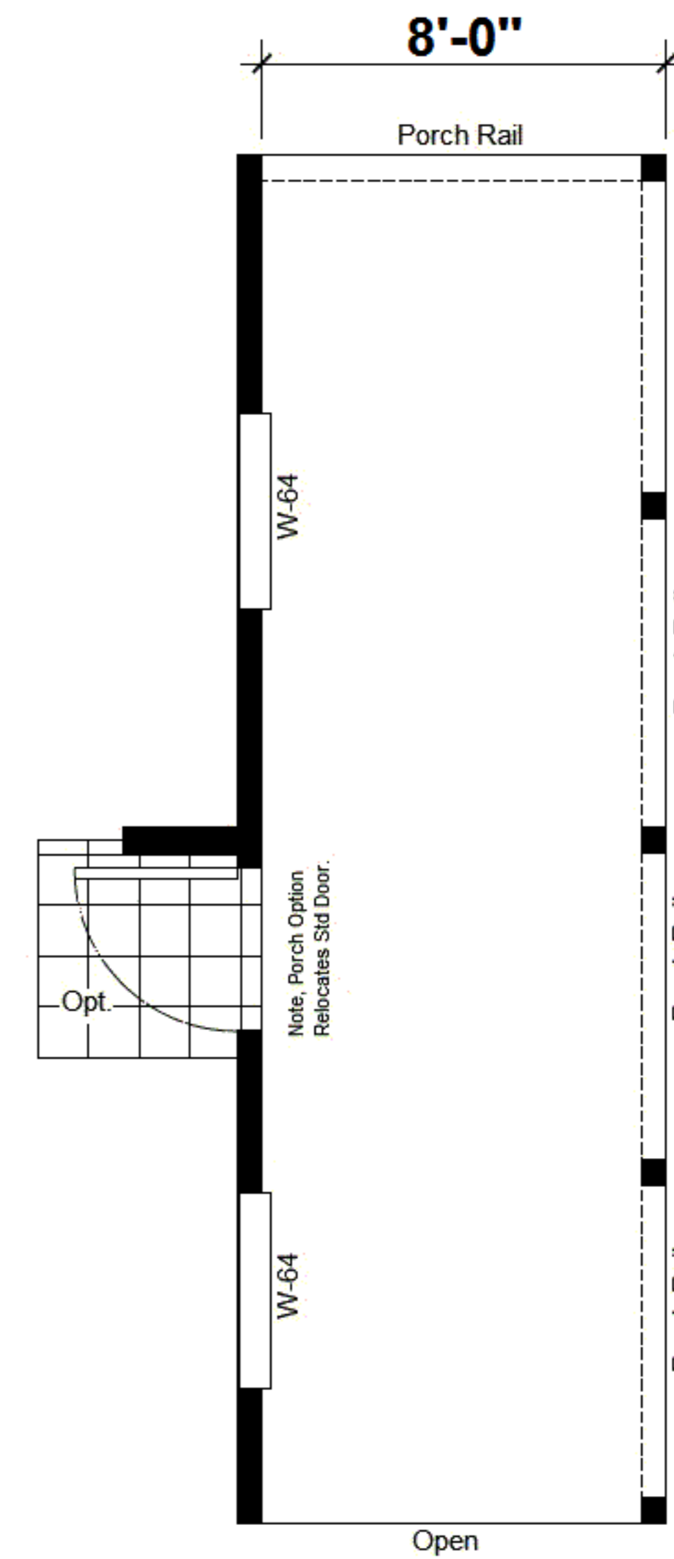
Opt. Porch
