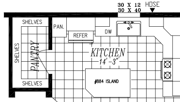
OPT. KITCHEN W/ PANTRY
