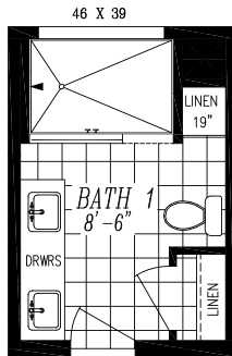
OPT. 48x72 TILE SHWR.
