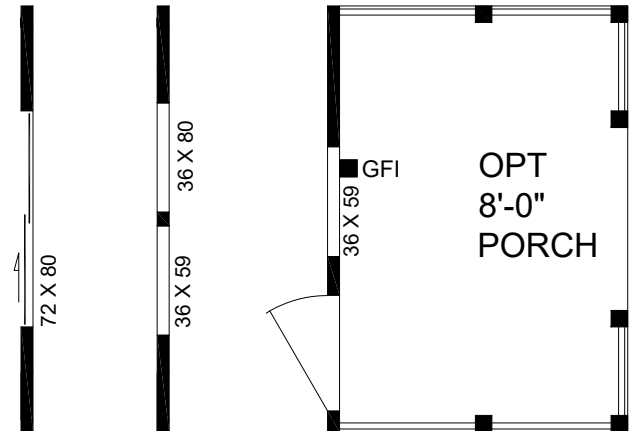
Optional Alternate Windows (Only Available W/ Sidewall Door Opt.) (N/A W/ Porch Opt.)
